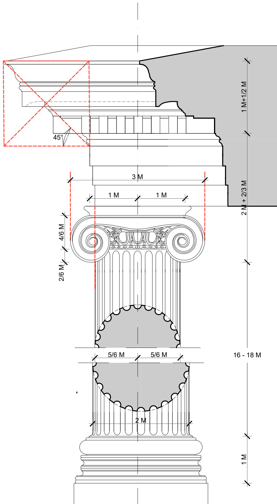
IONIC ORDER - ASIA MINOR TYPE
